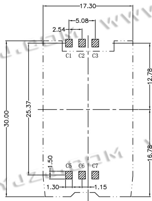
RECOMMENDED P. C. B LAYOUT COMPONENT SIDE (TOLERANCE \pm 0.05 )
